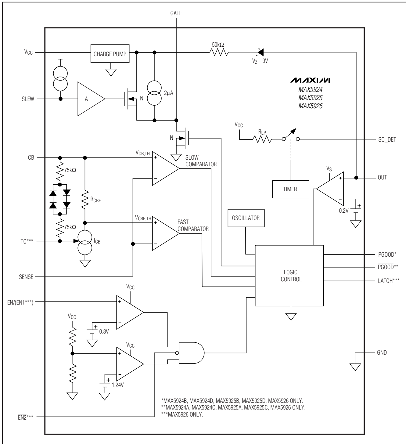
Figure 3. Functional Diagram
