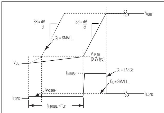
Figure 5. Startup Waveform
