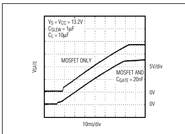
Figure 9. Impact of C_{GATE} on the V_{GATE} Waveform
