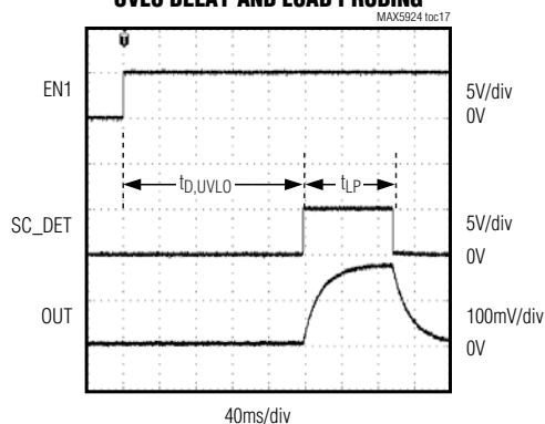
UVLO DELAY AND LOAD PROBING
