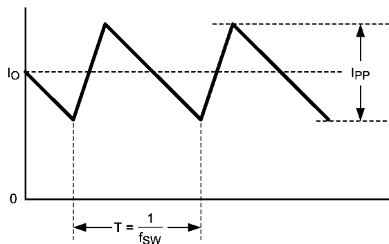
FIGURE 10. Inductor Current
