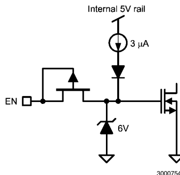
FIGURE 4. Enable Circuit
