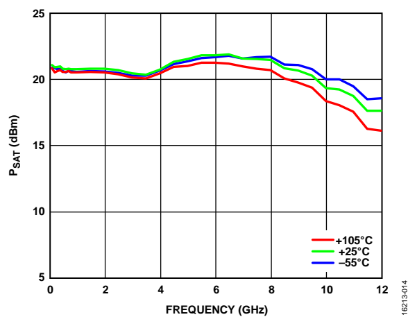
Figure 13. Saturation Power ( P_{SAT} ) vs. Frequency at Various Temperatures
