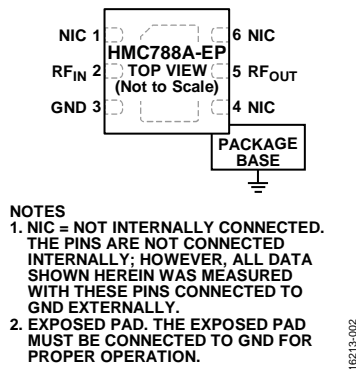
Figure 3. Pin Configuration
