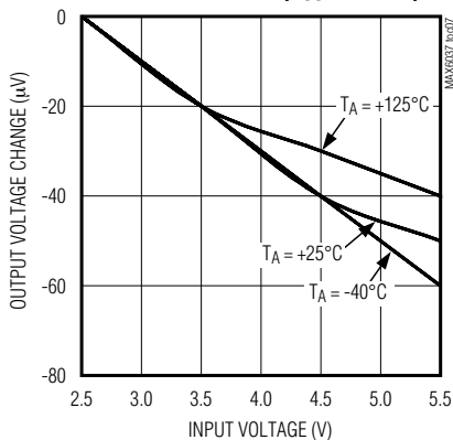
MAX6037_12 LINE REGULATION vs. TEMPERATURE ( V_{OUT} = 1.25V )
