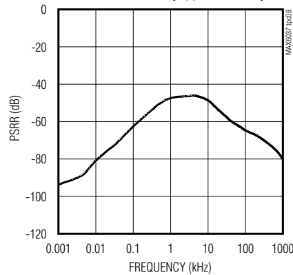
MAX6037_25 POWER-SUPPLY REJECTION RATIO vs. FREQUENCY ( V_{OUT} = 2.500V )
