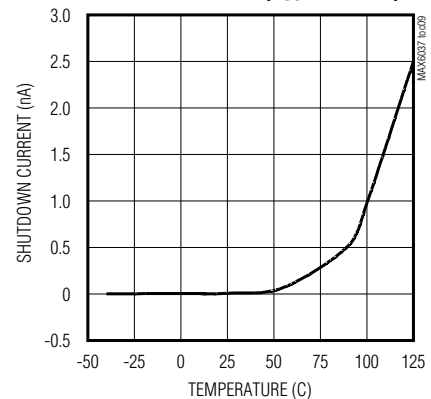
MAX6037_41 SHUTDOWN CURRENT vs. TEMPERATURE ( V_{OUT} = 4.096V )
