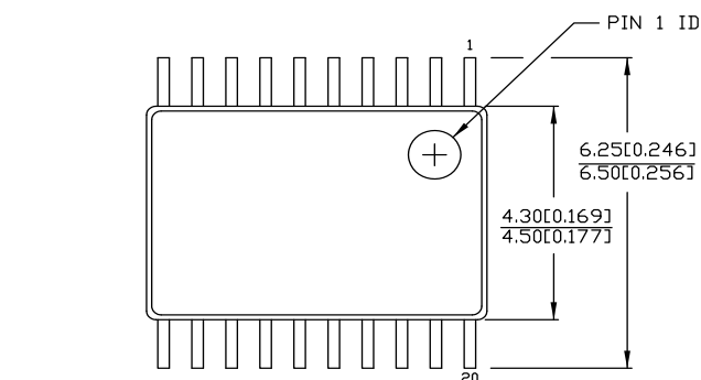
Figure 11. 20-pin TSSOP (4.40 mm Body) Z20.173/ZZ20.173 Package Outline, 51-85118
