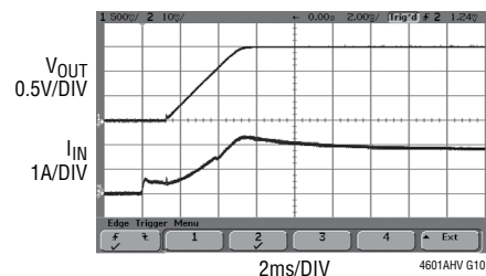
Start-Up, I_{OUT} = 12\text{A} (Resistive Load)
