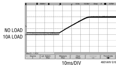
Start-Up, T_A = -55^\circ\text{C}
