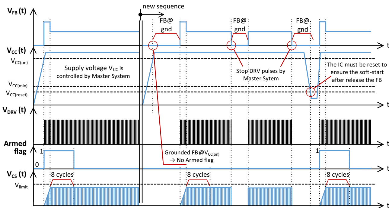
Figure 57. The Master system driving the controller by forcing the FB pin to ground.
