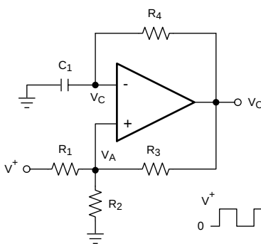
Figure 23. Square-Wave Oscillator
