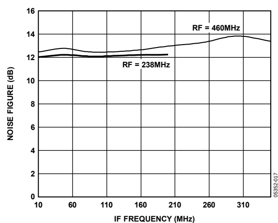
Figure 26. Noise Figure vs. IF Frequency
