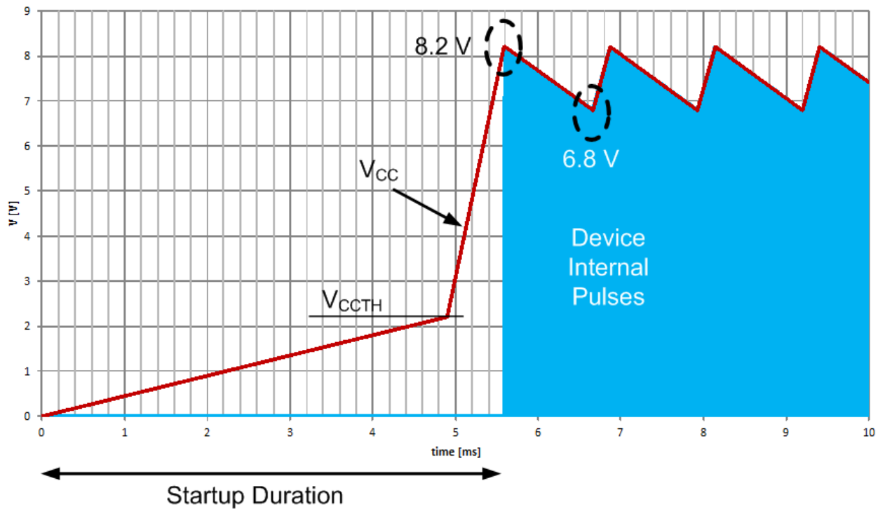
Figure 25. The Charge/Discharge Cycle Over a 1 \mu F V_{CC} Capacitor
