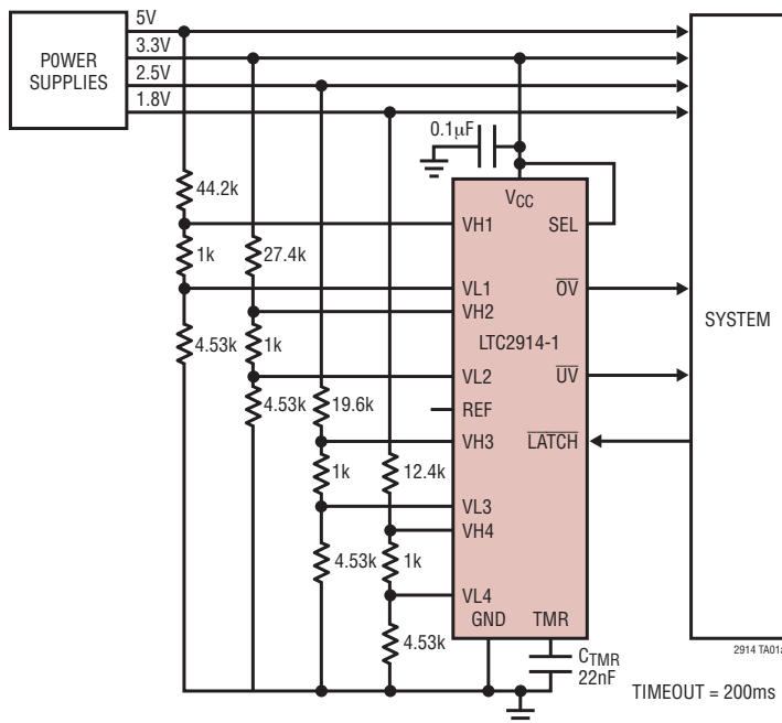
Quad UV/OV Supply Monitor, 10% Tolerance, 5V, 3.3V, 2.5V, 1.8V
