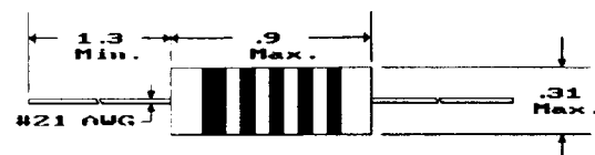
L Series Dimensions
