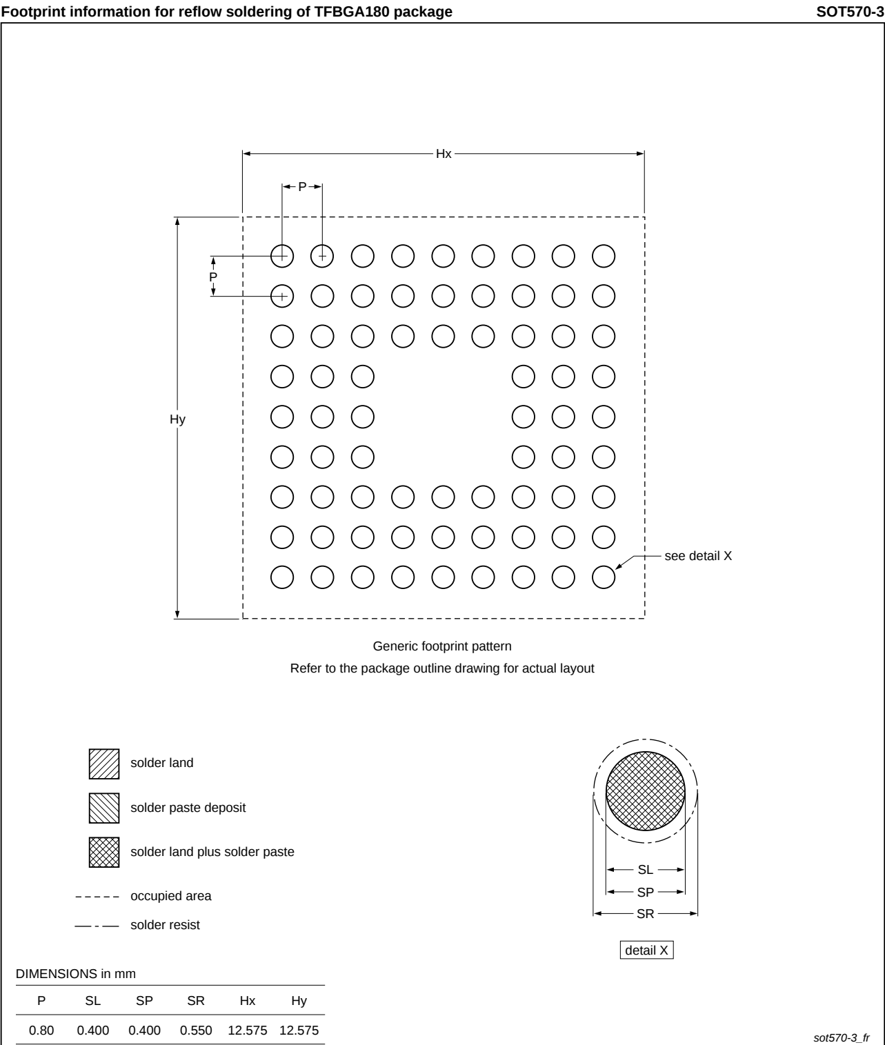
Fig 53. Reflow soldering of the TFBGA180 package
