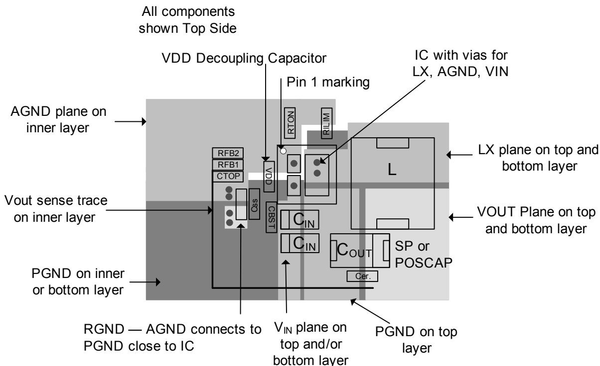
Figure 15 — PCB Layout
