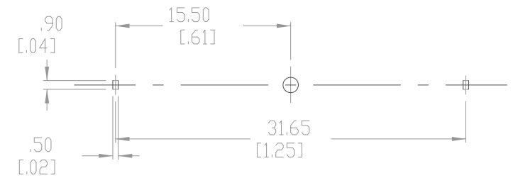
PCB LAYOUT
