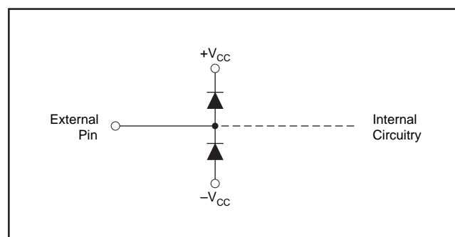
FIGURE 17. Internal ESD Protection.
