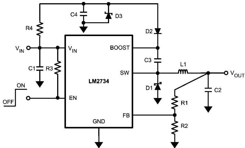
FIGURE 10. V_{\text{BOOST}} Derived from V_{\text{SHUNT}} 18V to 1.5V/1A
