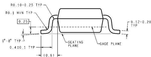
6-Lead SOT23 Package NS Package Number MK06A
