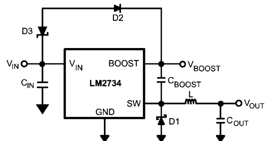
FIGURE 4. Zener Reduces Boost Voltage from V_{\text{IN}}
