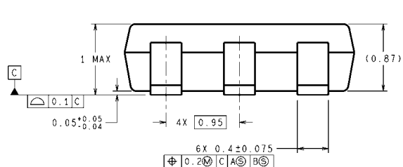
6-Lead SOT23 Package NS Package Number MK06A
