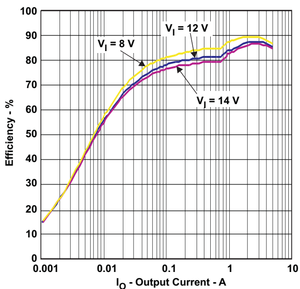
Figure 54. 1.05-V Efficiency
