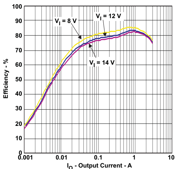
Figure 62. 1.2-V Efficiency
