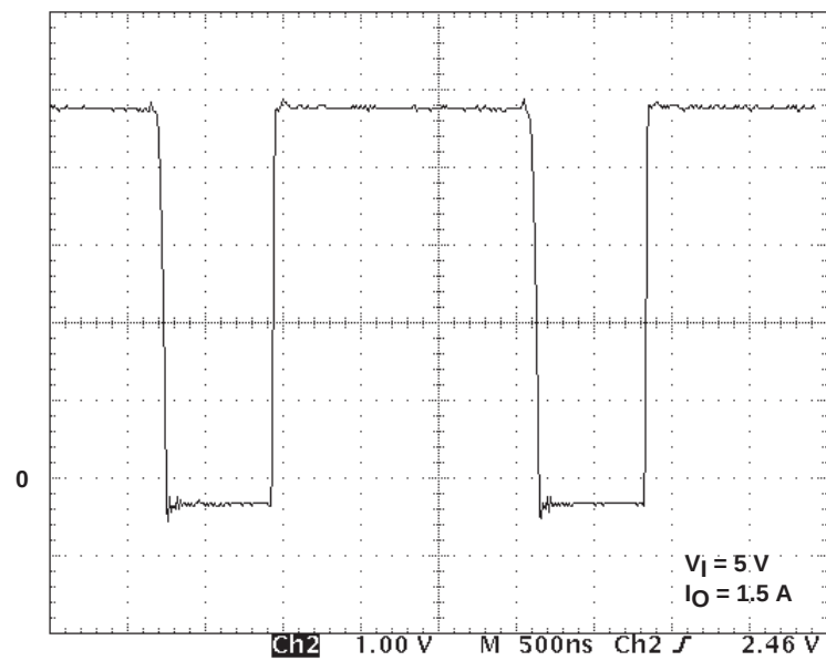
Figure 1–12. VDRAIN-To-GND Voltage
