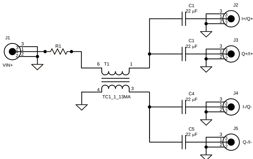
Figure 2. TC1-DESIQ-SBB Schematic
