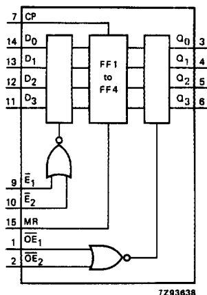
Fig.4 Functional diagram.
