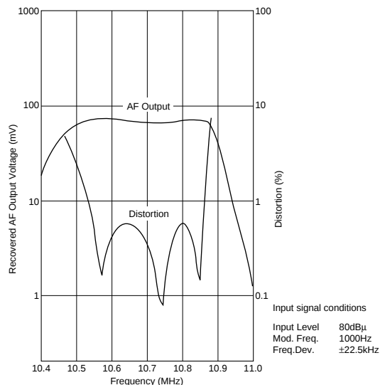
Frequency Characteristics
