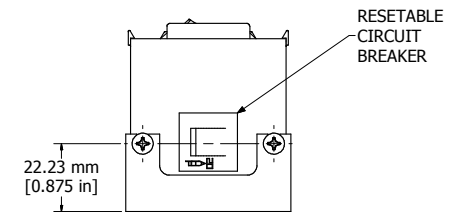
ASSEMBLY - VIEW FROM END
