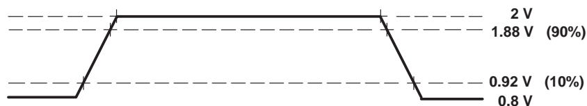
Figure 7. TTL-Level Inputs
