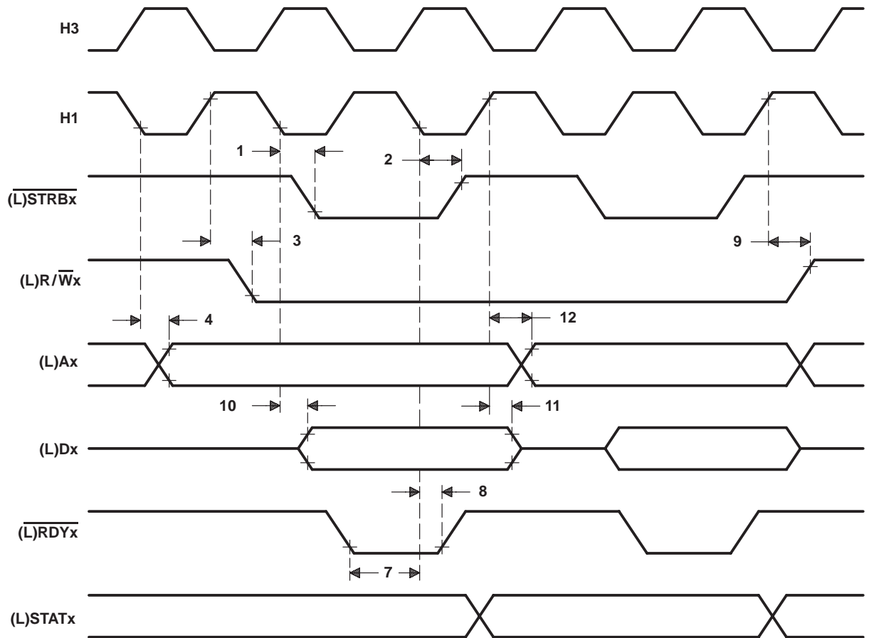
Figure 11. Memory-Write-Cycle Timing [ \overline{(L)STRBx} = 0 ]
