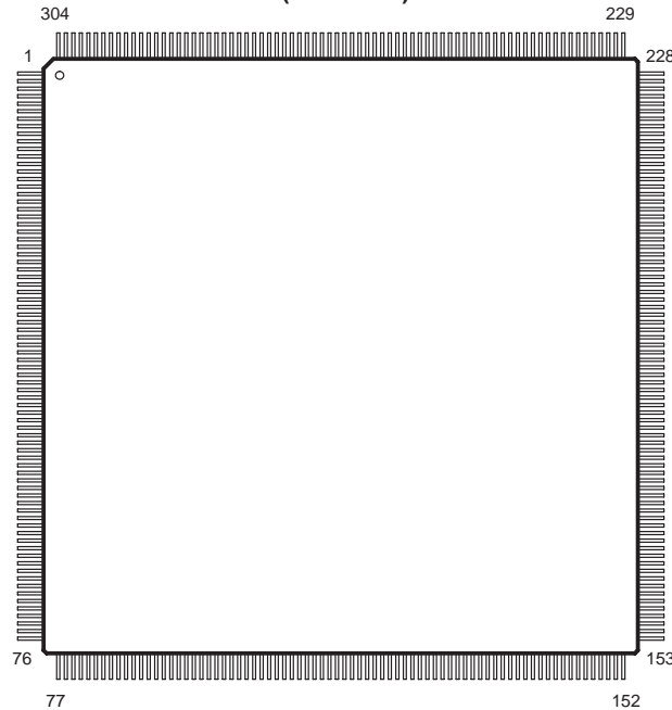
304-PIN PDB PLASTIC QUAD FLATPACK (TOP VIEW)
