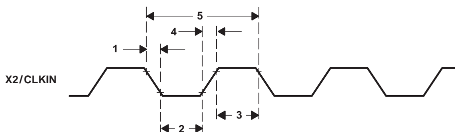
Figure 8. X2/CLKIN Timing
