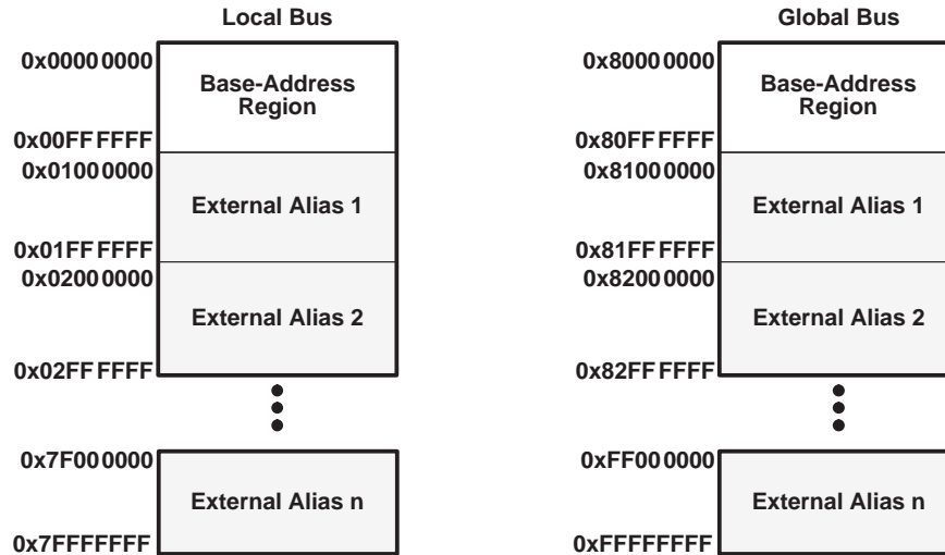
Figure 2. Memory Alias
