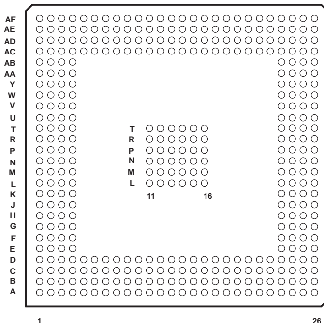
388-PIN GFW BALL GRID ARRAY (BOTTOM VIEW)
