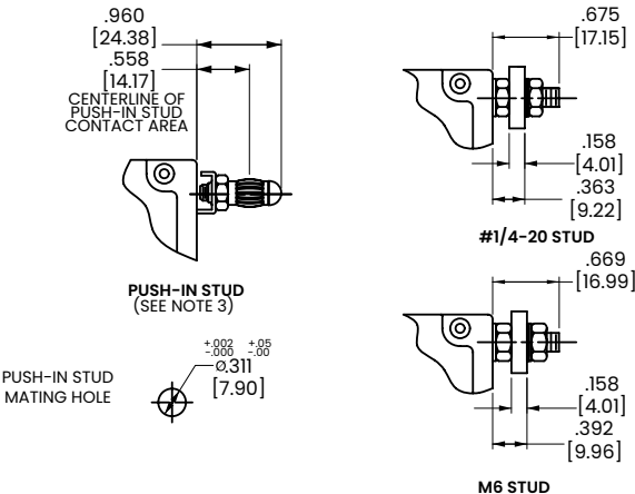
TERMINAL DETAILS
