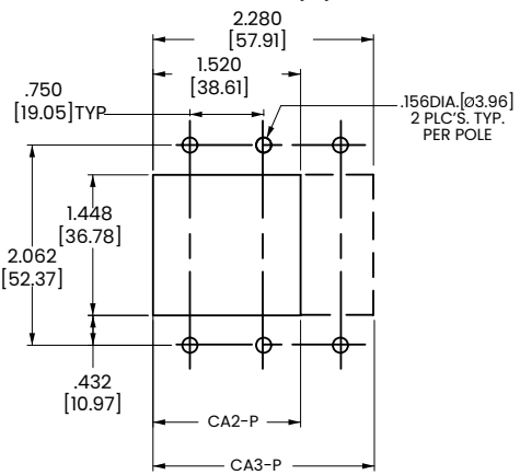
PANEL CUT-OUT DETAIL
