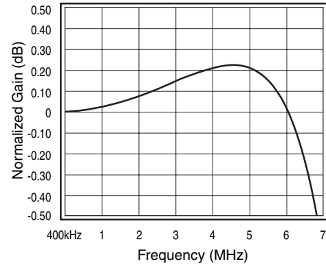
Figure 2. SD Gain Flatness
