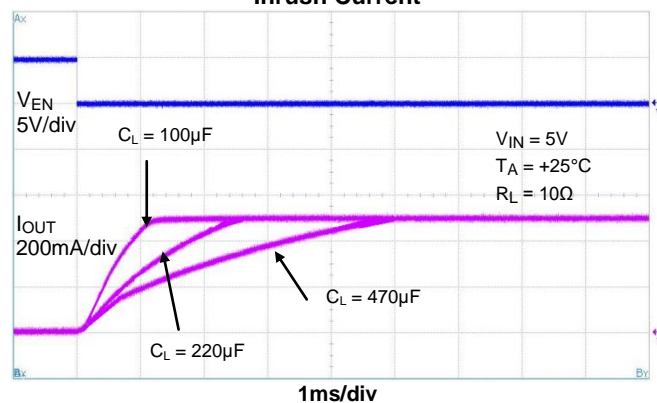
Inrush Current
