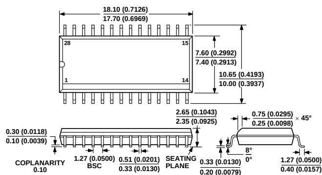
CONTROLLING DIMENSIONS ARE IN MILLIMETERS; INCH DIMENSIONS (IN PARENTHESES) ARE ROUNDED-OFF MILLIMETER EQUIVALENTS FOR REFERENCE ONLY AND ARE NOT APPROPRIATE FOR USE IN DESIGN Figure 26. 28-Lead Standard Small Outline Package [SOIC_W] Wide Body (RW-28) Dimensions shown in millimeters and (inches)
