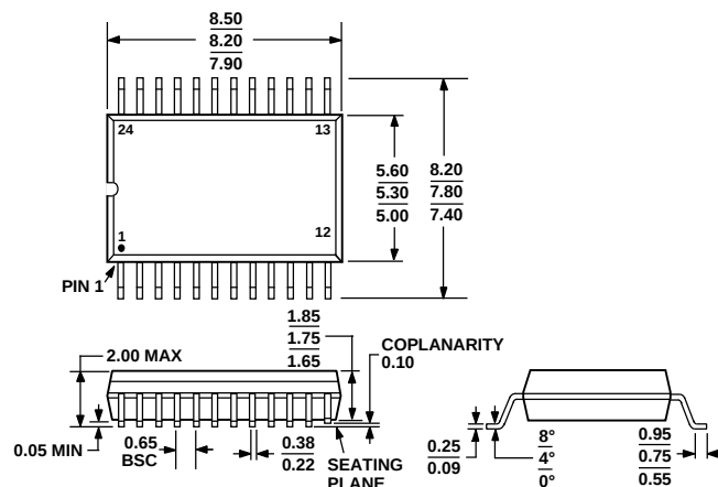
Figure 25. 24-Lead Shrink Small Outline Package [SSOP] (RS-24) Dimensions shown in millimeters
