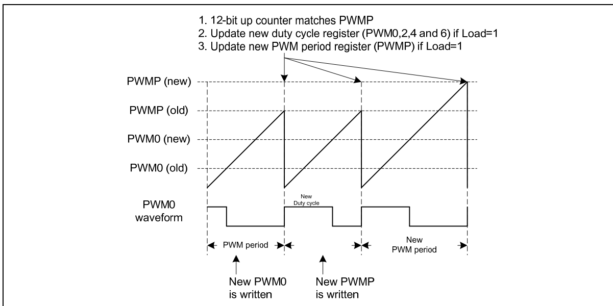
Figure 14-16: Edge-Aligned PWM
