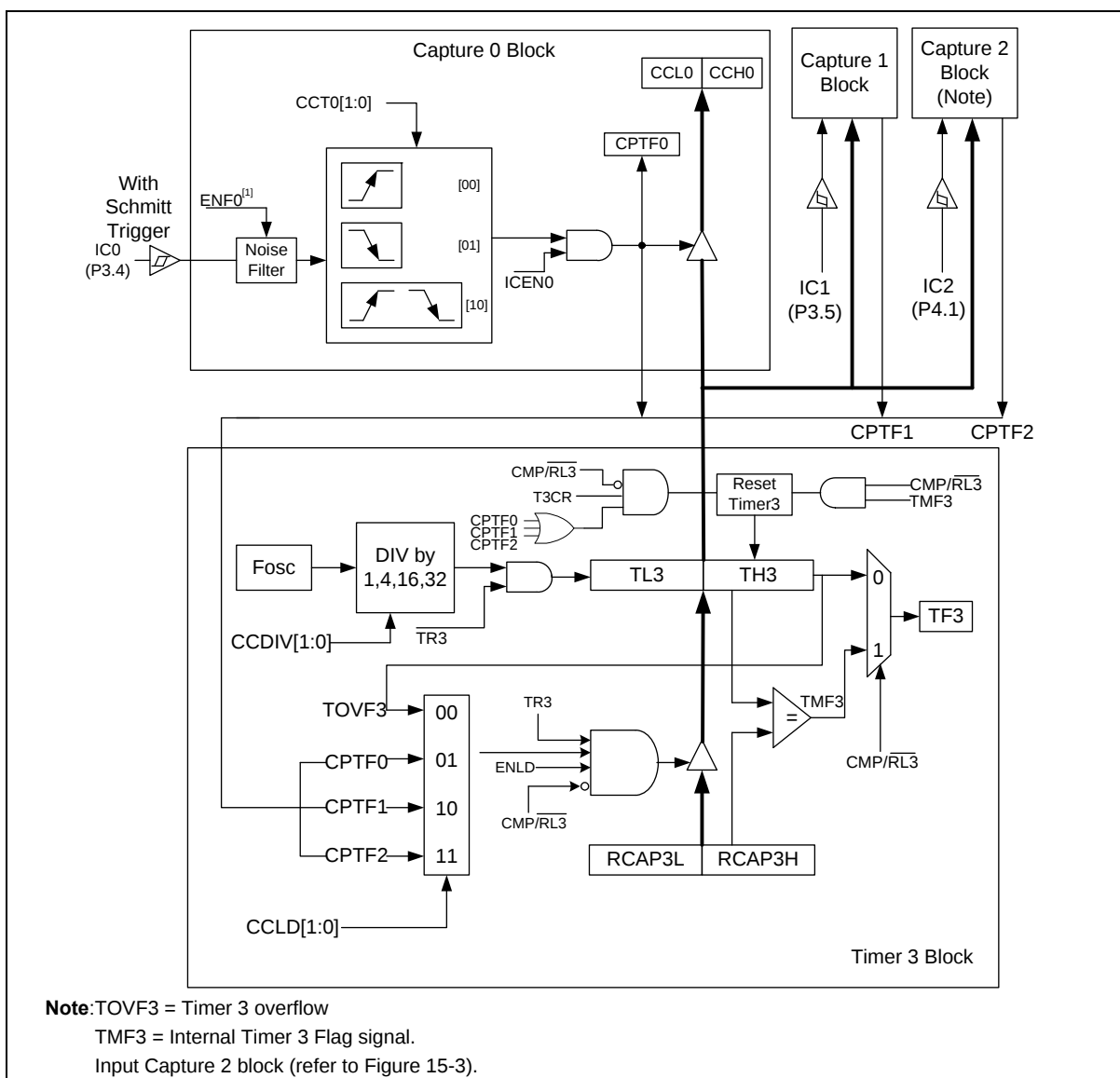
Figure 15-2: Timer3/Capture/Compare/Reload modules
