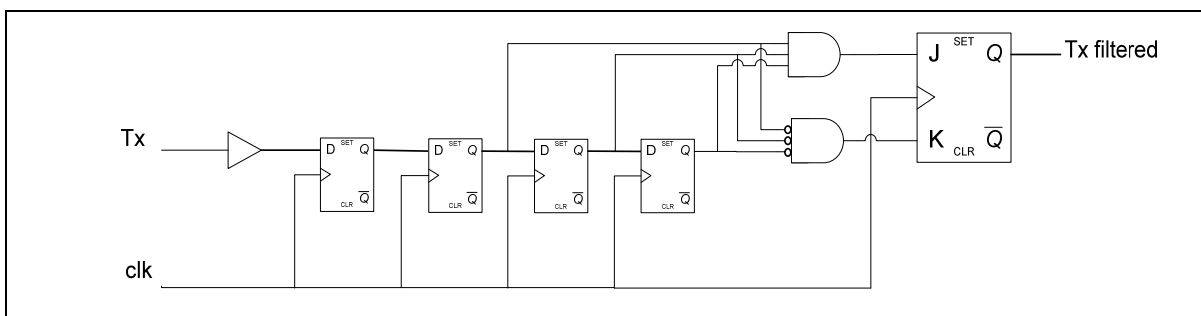
Figure 15-1: Noise Filter
