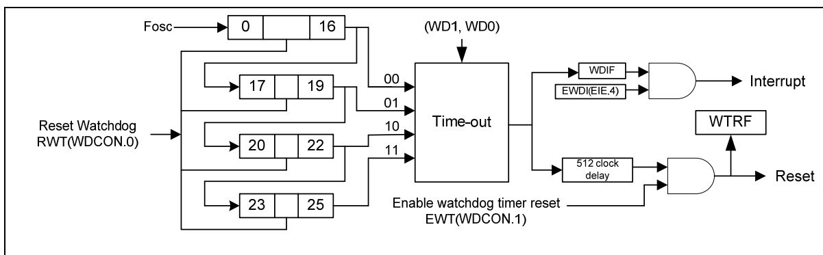
Figure 13-1: Watchdog Timer
