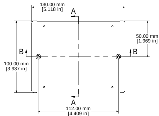
ASSEMBLY - BOTTOM
