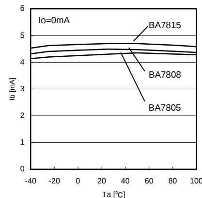
Fig.23 T_a - I_b
