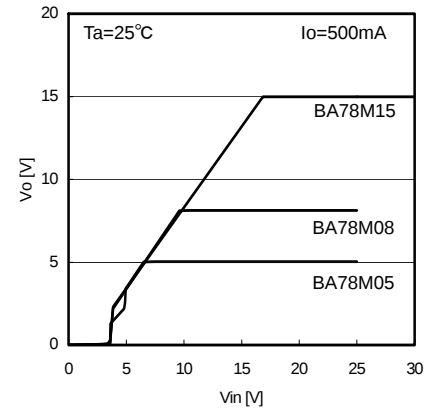
Fig.3 Line Regulation ( I_o=500\text{mA} )
