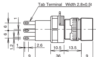
Solder/Tab Terminal
