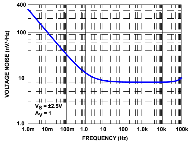
FIGURE 51. SIMULATED INPUT NOISE VOLTAGE
