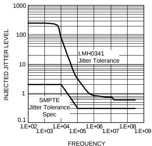
Figure 8. Jitter Tolerance Curve
