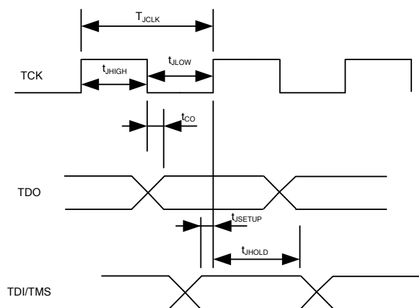
Figure 17. JTAG timing
