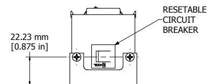
ASSEMBLY - VIEW FROM END
