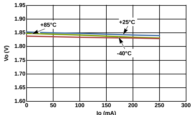
FIGURE 5. LOAD REGULATION vs TEMPERATURE ( V_{OUT} = 1.85\text{V} )
