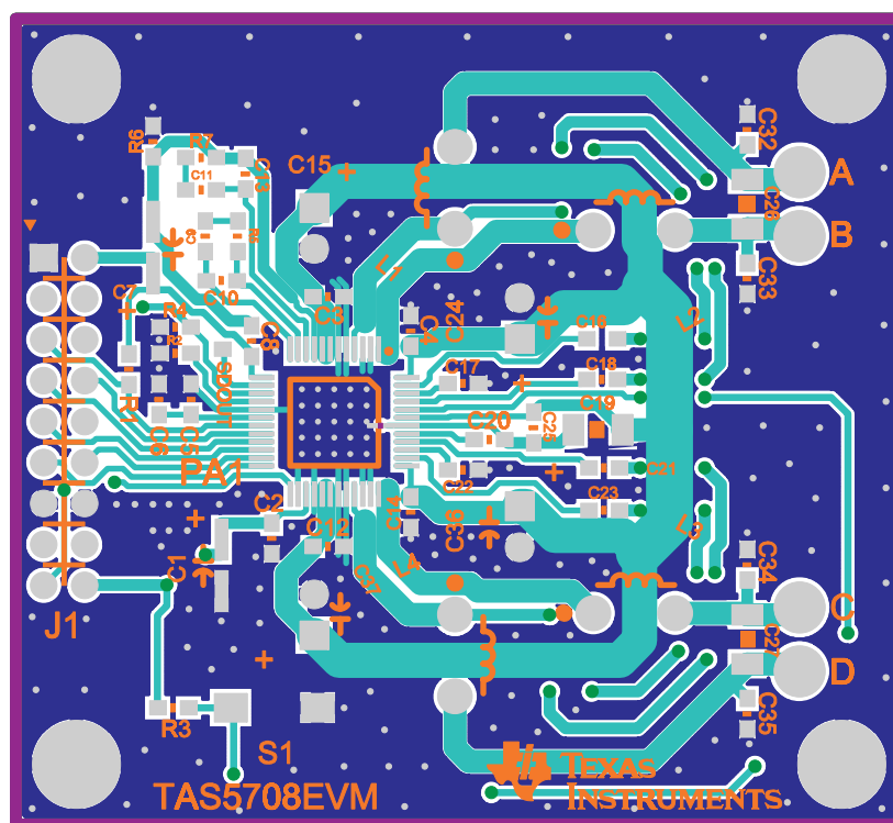
Figure 15. TAS5708(TAS5710)EVM Top Composite Assembly
