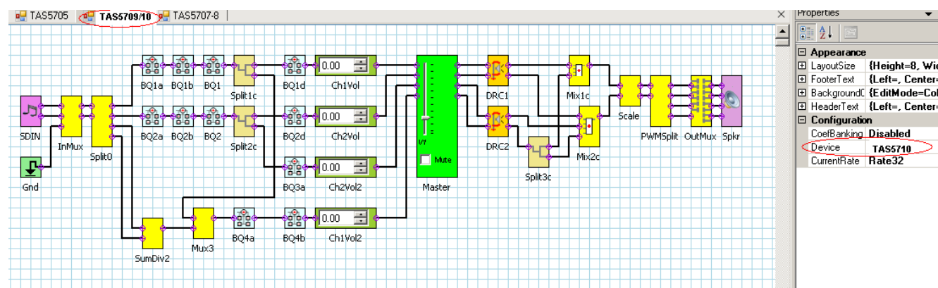
Figure 7. Process Flow for TAS5710 UG
