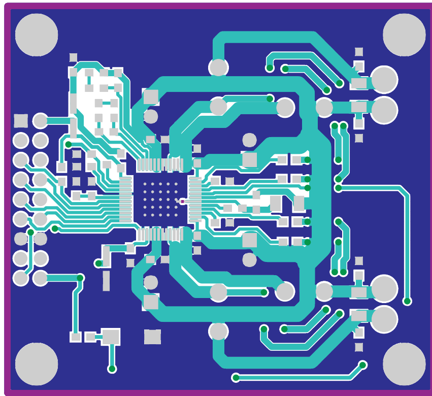
Figure 16. TAS5708(TAS5710)EVM Top Copper Assembly
