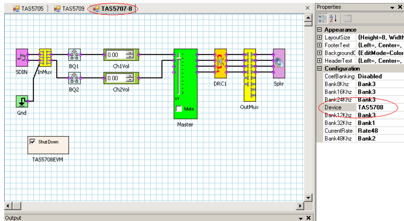
Figure 6. Process Flow for TAS5708 UG
