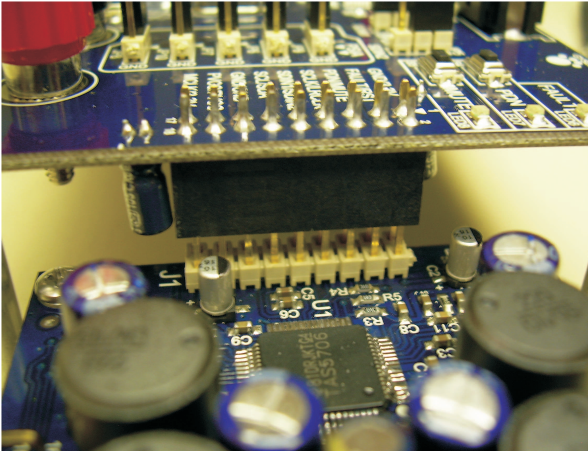
Figure 4. Connecting TAS5708(TAS5710)EVM to MC57xxPSIA
