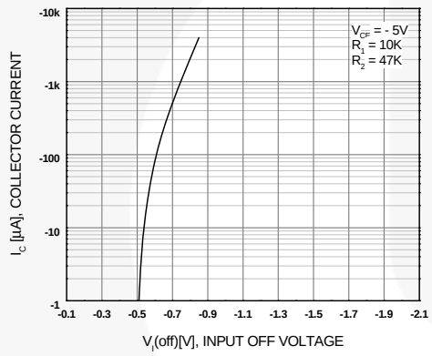
Figure 3. Input-Off Voltage
