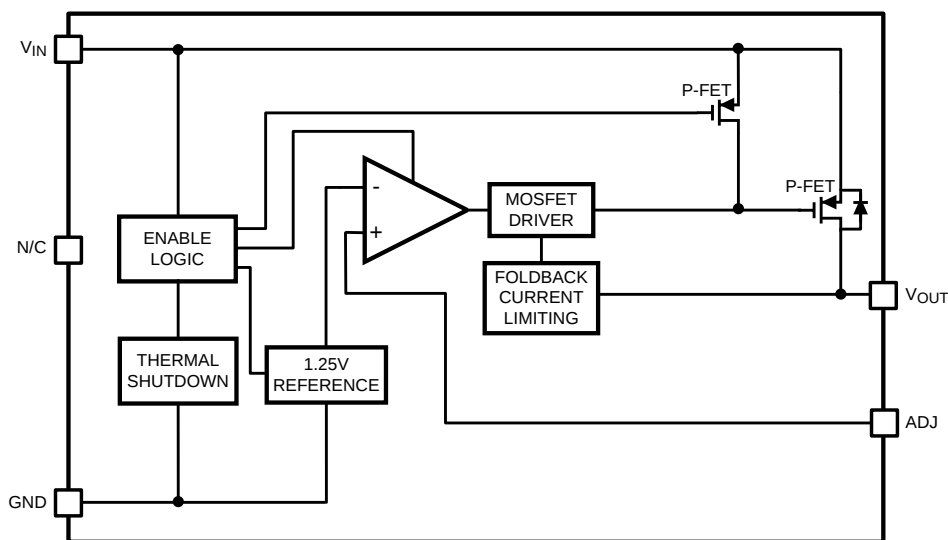
Figure 4. LP38691-ADJ Functional Diagram (WSO)
