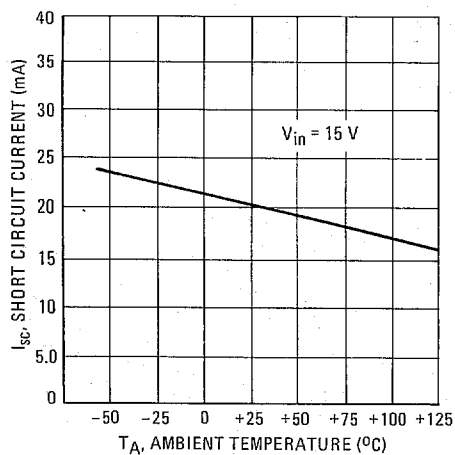
FIGURE 8 – SHORT CIRCUIT CURRENT versus TEMPERATURE
