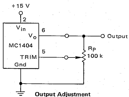
FIGURE 10 – OUTPUT TRIM CONFIGURATION
