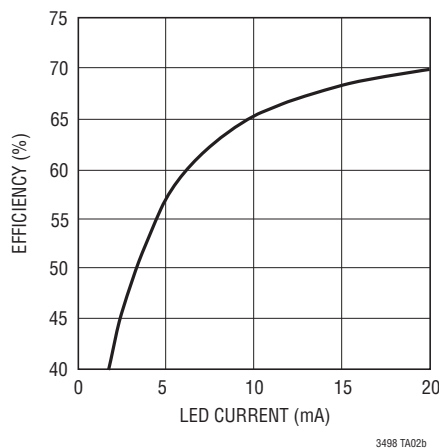
LED Efficiency VIN = 3.6V, 2 LEDs
