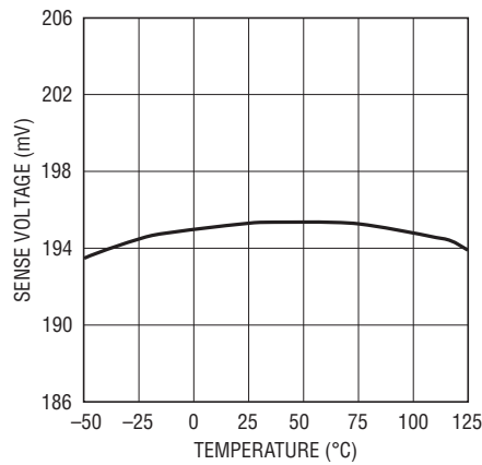
Sense Voltage (V CAP1 - V LED1 ) vs Temperature
