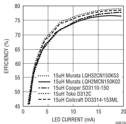
Figure 2. Efficiency Comparison of Different Inductors
