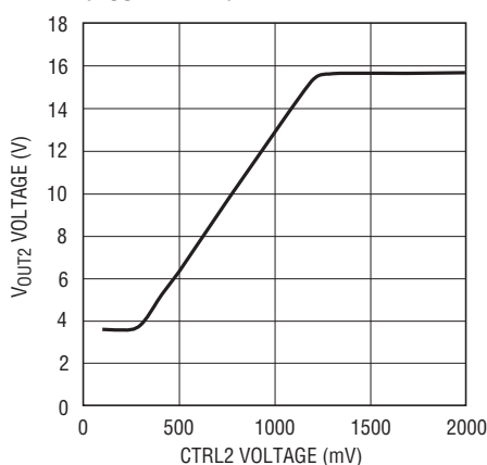
V OUT2 vs V CTRL2 (V OUT2 = 16V)
