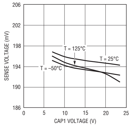
Sense Voltage (V CAP1 - V LED1 ) vs V CAP1
