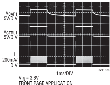
LED Transient Response
