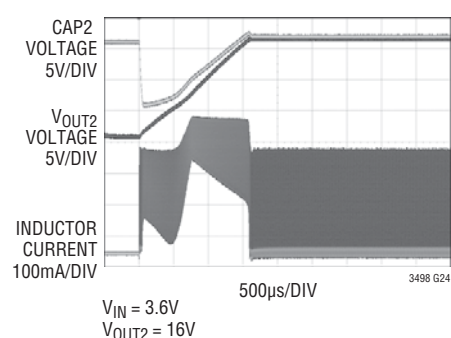
OLED Switching Waveforms During Start-Up
