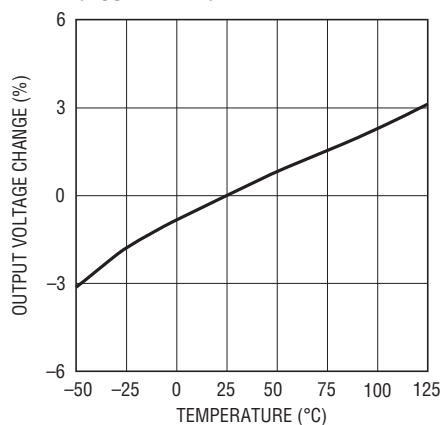
V OUT2 vs Temperature (V OUT2 = 16V)
