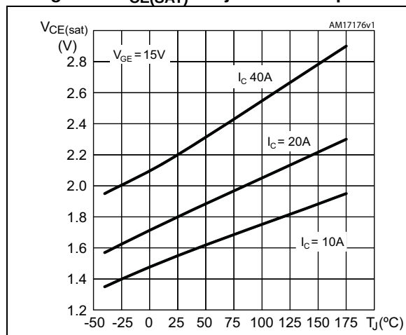
Figure 6. V_{CE(SAT)} vs. junction temperature
