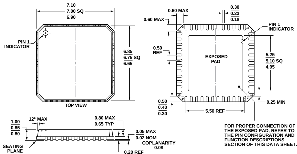
COMPLIANT TO JEDEC STANDARDS MO-220-VKGD-2 Figure 37. 48-Lead Lead Frame Chip Scale Package [LFCSP_VQ] 7 mm x 7 mm Body, Very Thin Quad (CP-48-1)
