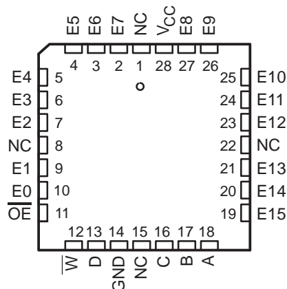
SN54AS250A . . . FK PACKAGE (TOP VIEW)
