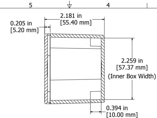
SECTION K-K End View of Assembly
