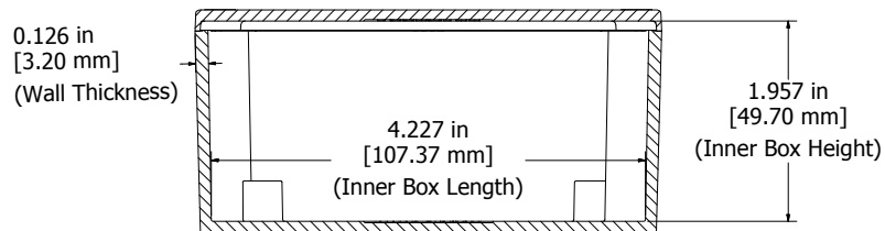
SECTION J-J Side View of Assembly
