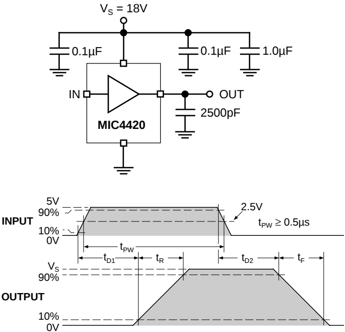
Figure 1b. Noninverting Driver Switching Time
