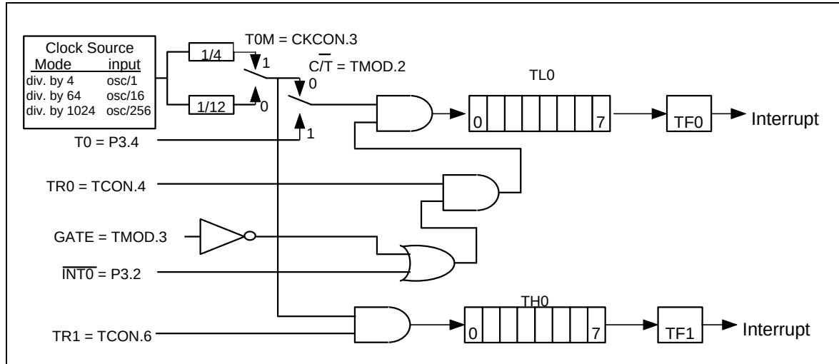
Figure 13. Timer/Counter 0 Mode 3
