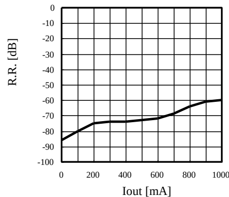
■AP1154ADL50 Iout=1mA~1A , f=1kHz
