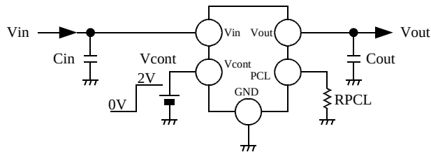
Measurement circuit
