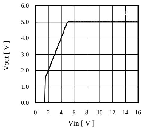
■ Line Regulation (AP1154ADL50)
