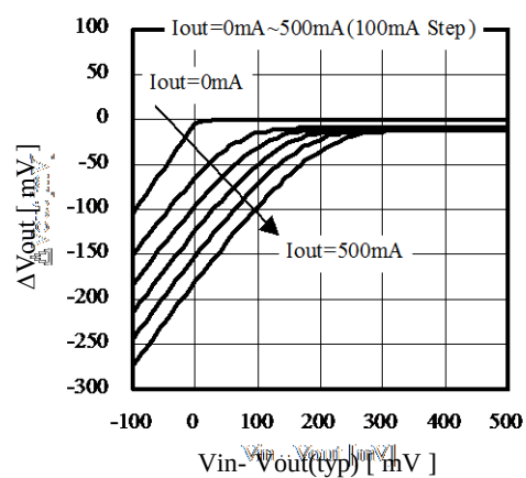
■ \Delta V_{\text{out}} vs \Delta V_{\text{in}} (AP1154ADL50)
