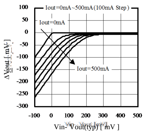
■ \Delta V_{\text{out}} vs \Delta V_{\text{in}} (AP1154ADL25)
