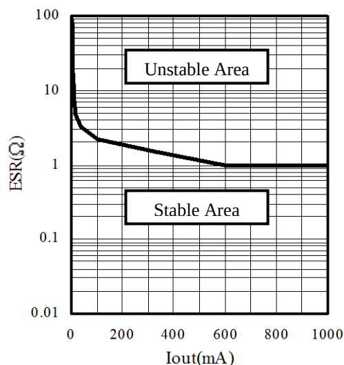
Figure 2. Stable operation area ( C_{\text{Out}} \geq 0.47\mu\text{F} )
