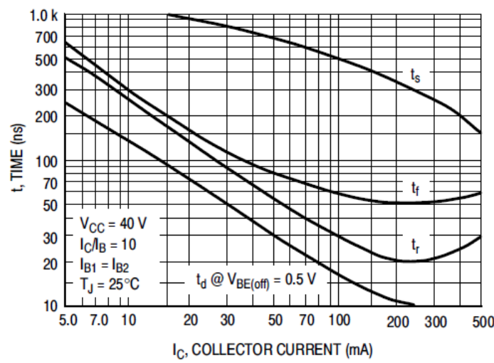
Fig.3 Switching Time
