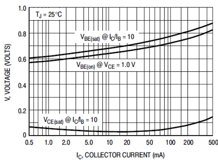
Fig.5 ON Voltages
