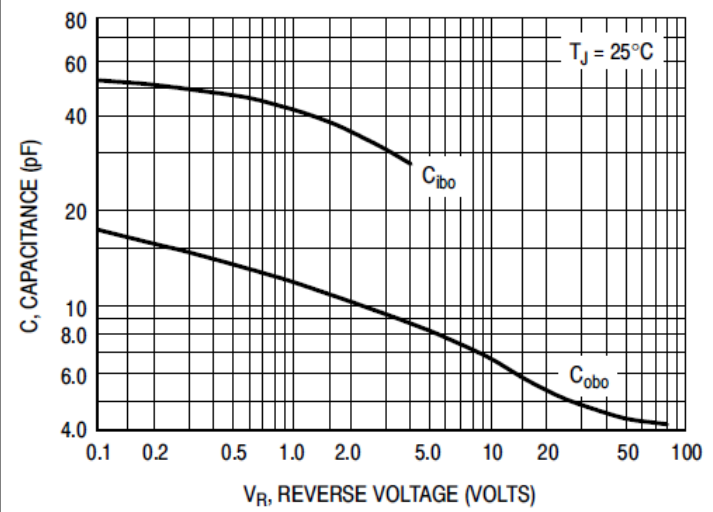
Fig.2 Capacitance
