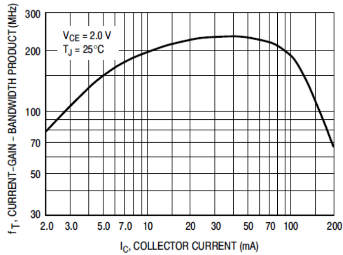
Fig.1 Current-Gain—Bandwidth Product
